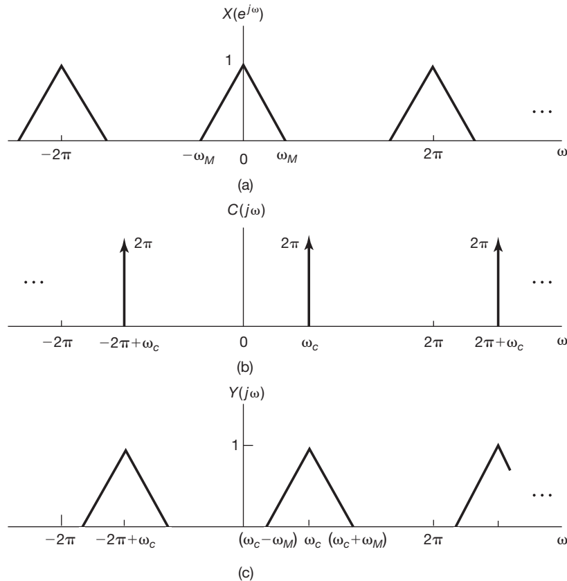
Figura 8.41 (a) Espectro de x[n] . (b) Espectro de c[n] = e^{j\omega_c n} . (c) Espectro de y[n] = x[n]c[n] .
