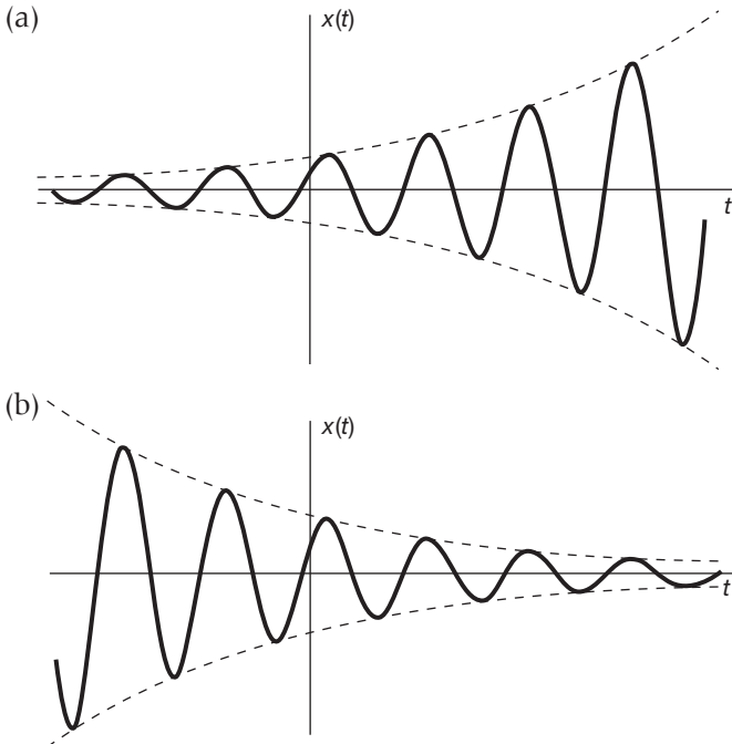
Figura 1.23 (a) Sinal senoidal crescente x(t) = Ce^{rt} \cos(\omega_0 t + \theta) , r > 0 ; (b) senoidal decrescente x(t) = Ce^{rt} \cos(\omega_0 t + \theta) , r < 0 .
